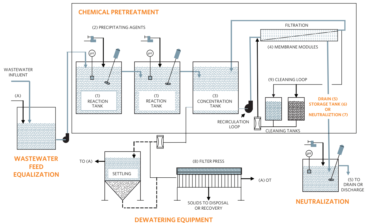
Microfiltration Wastewater Treatment System
