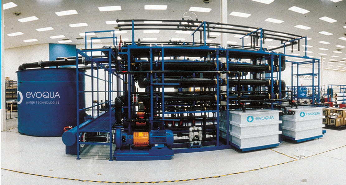
Memtek® EFC-Series Microfiltration System
