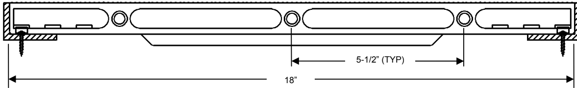
SIDE VIEW – 18"
