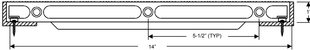
SIDE VIEW – 14"
