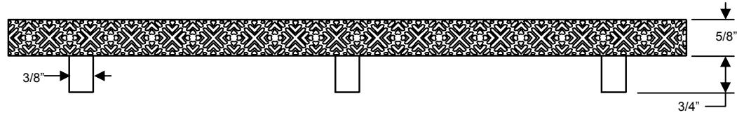
PLAN VIEW – 14"
