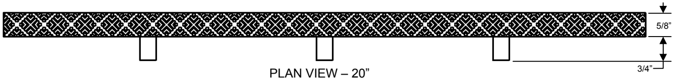
PLAN VIEW – 20"
